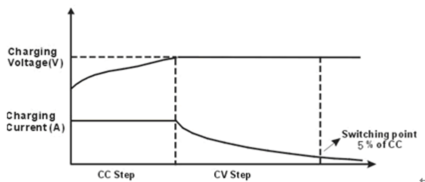
Charging Curve
